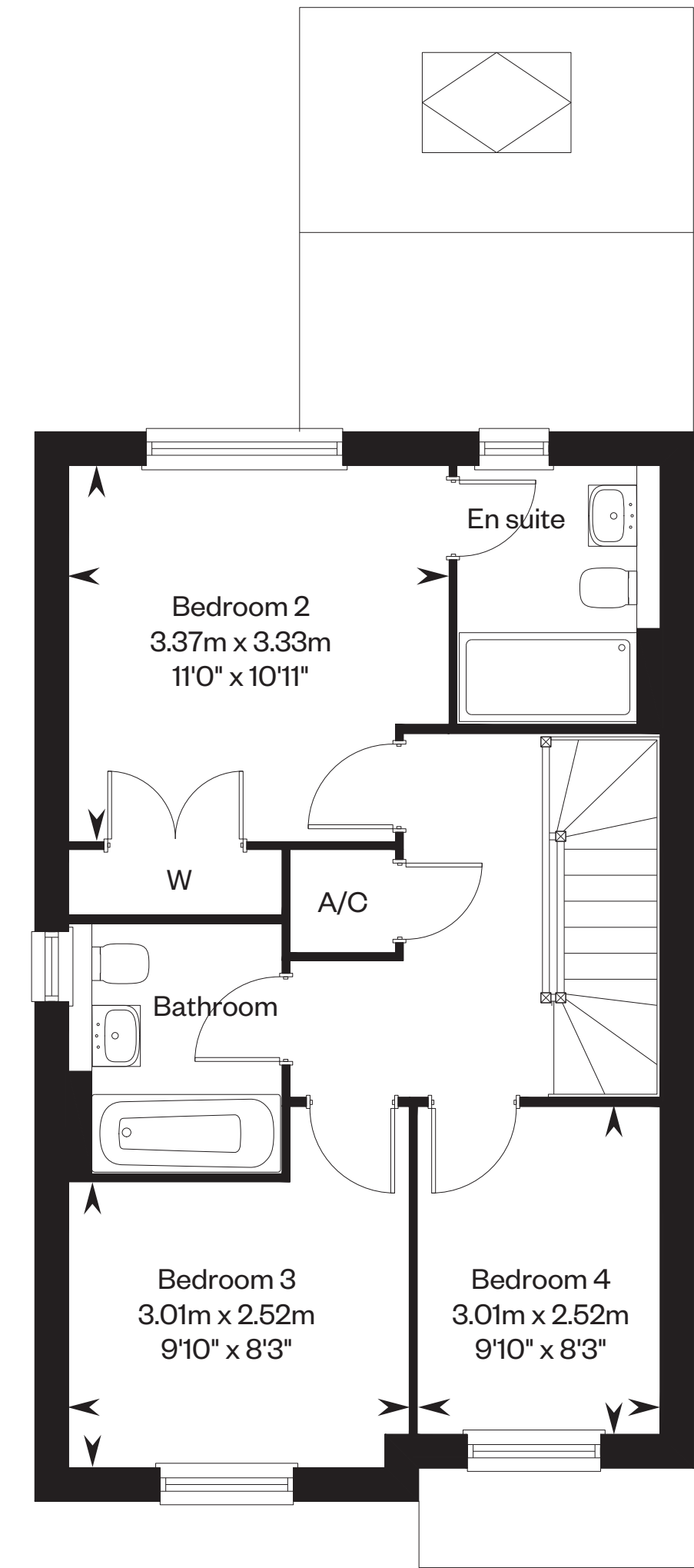
Second floor
