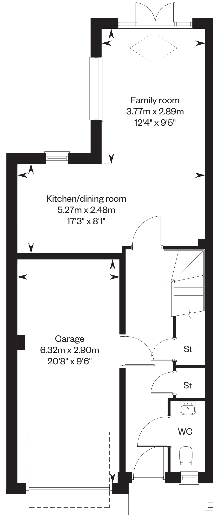
Ground floor
